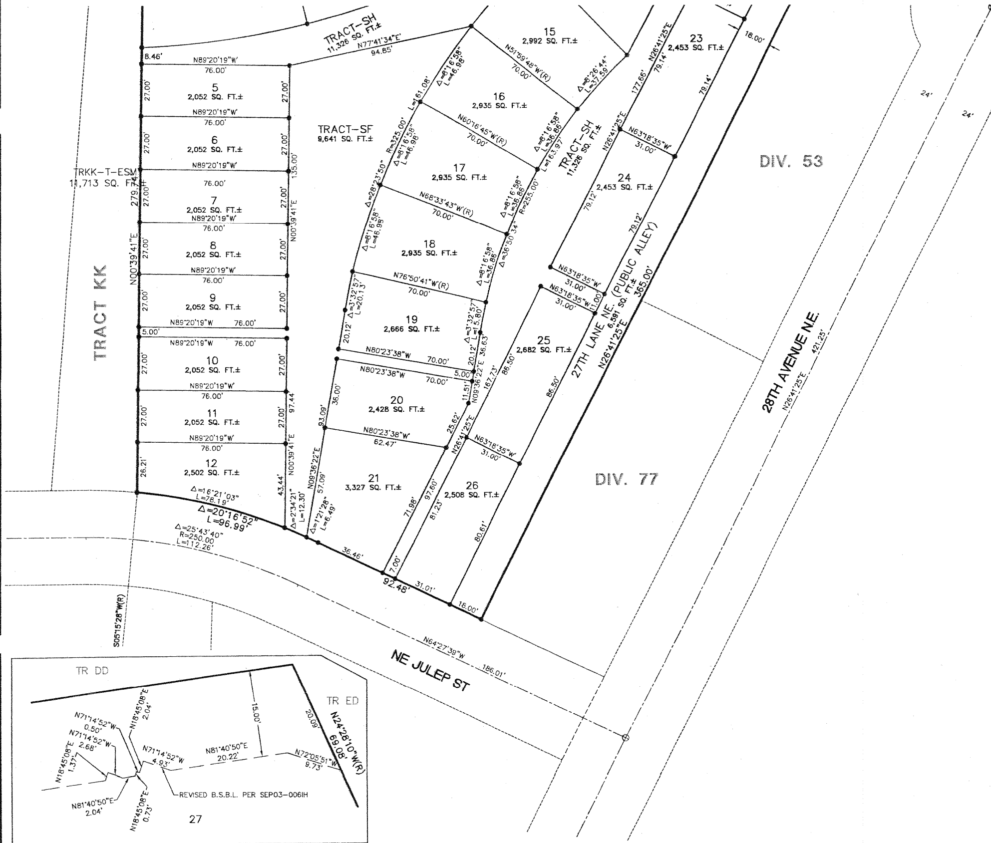
DETAIL "B" SCALE 1"=10'
