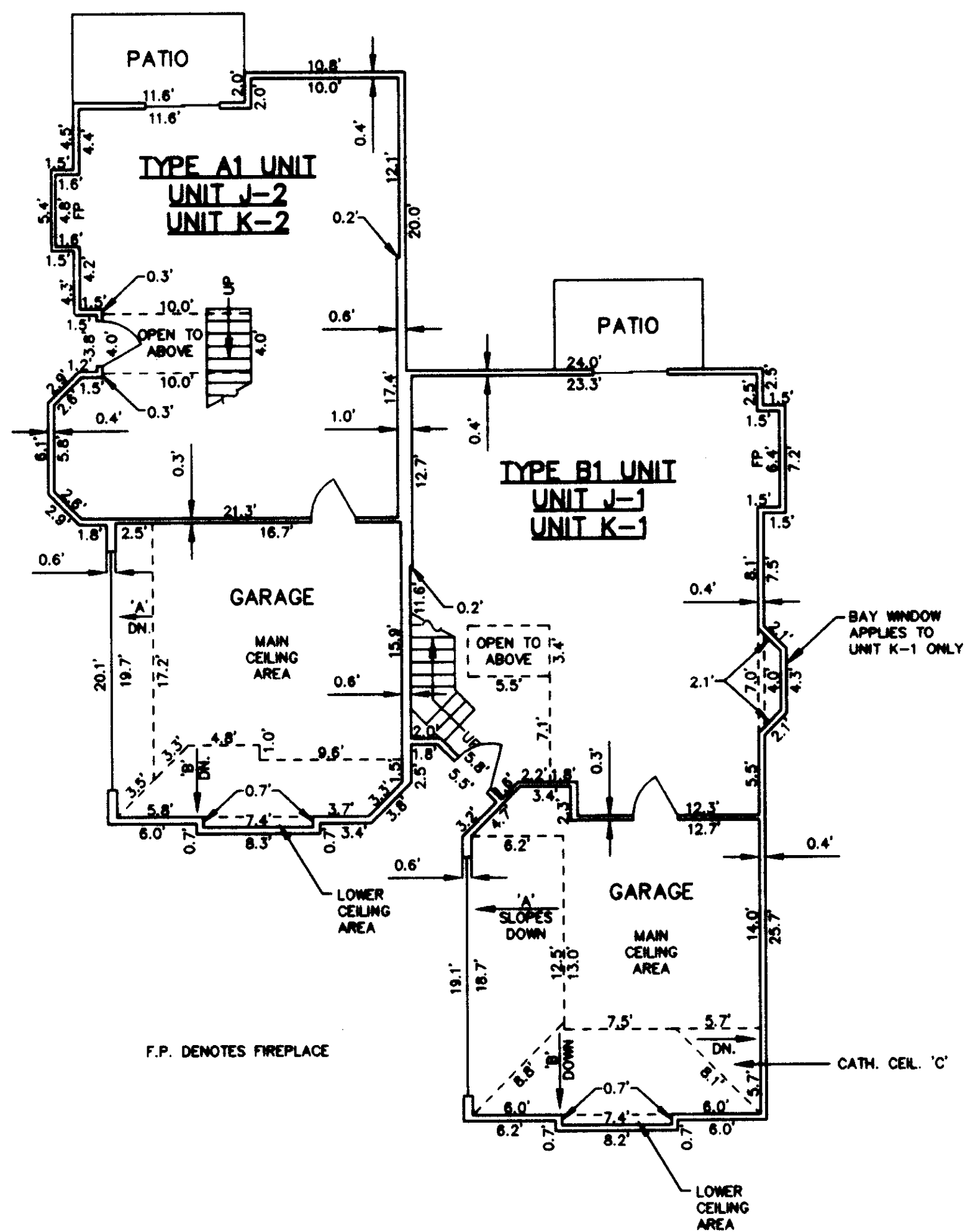
BUILDING TYPE 1
