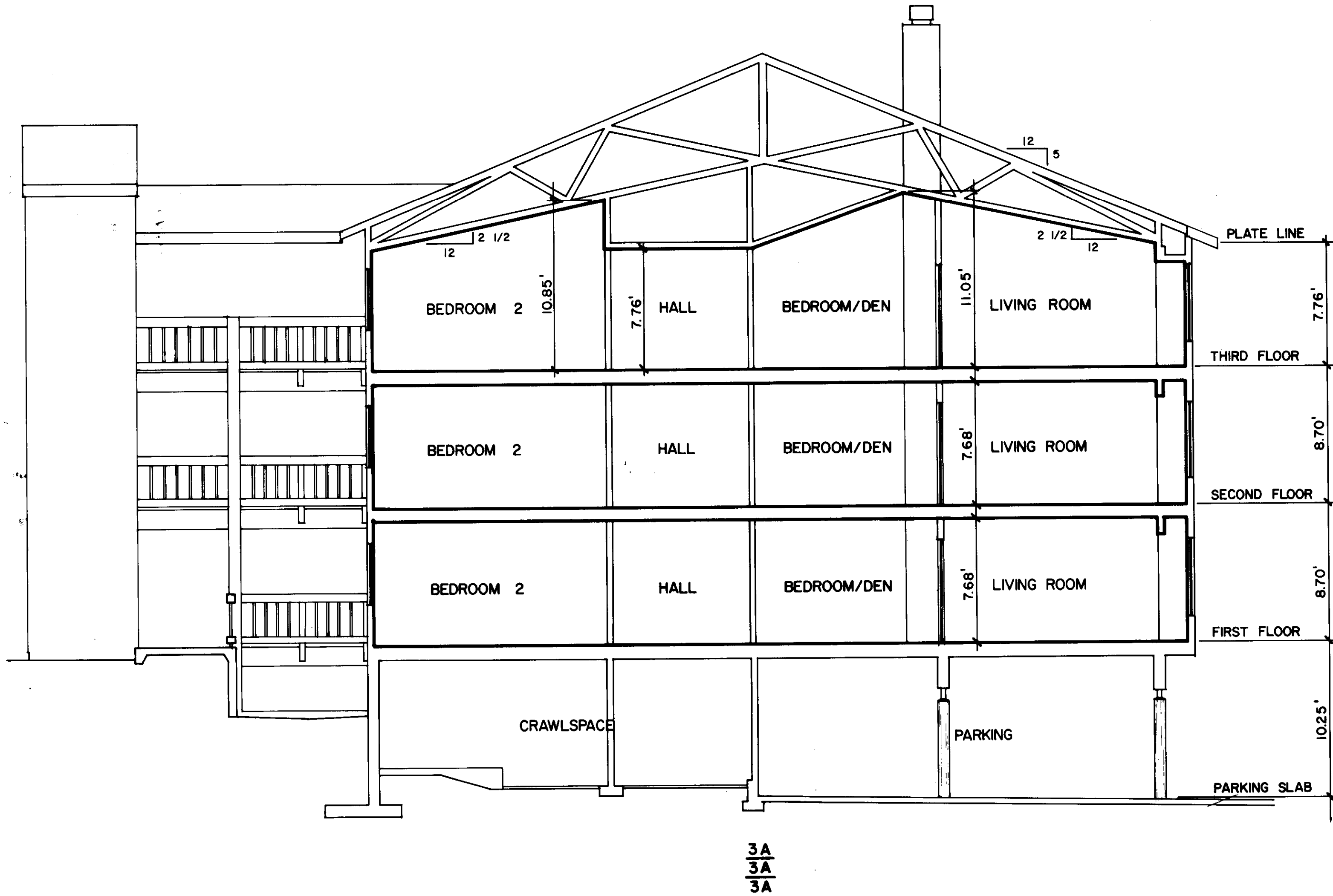
BUILDING SECTION B-B 3/16" = 1'-0"
