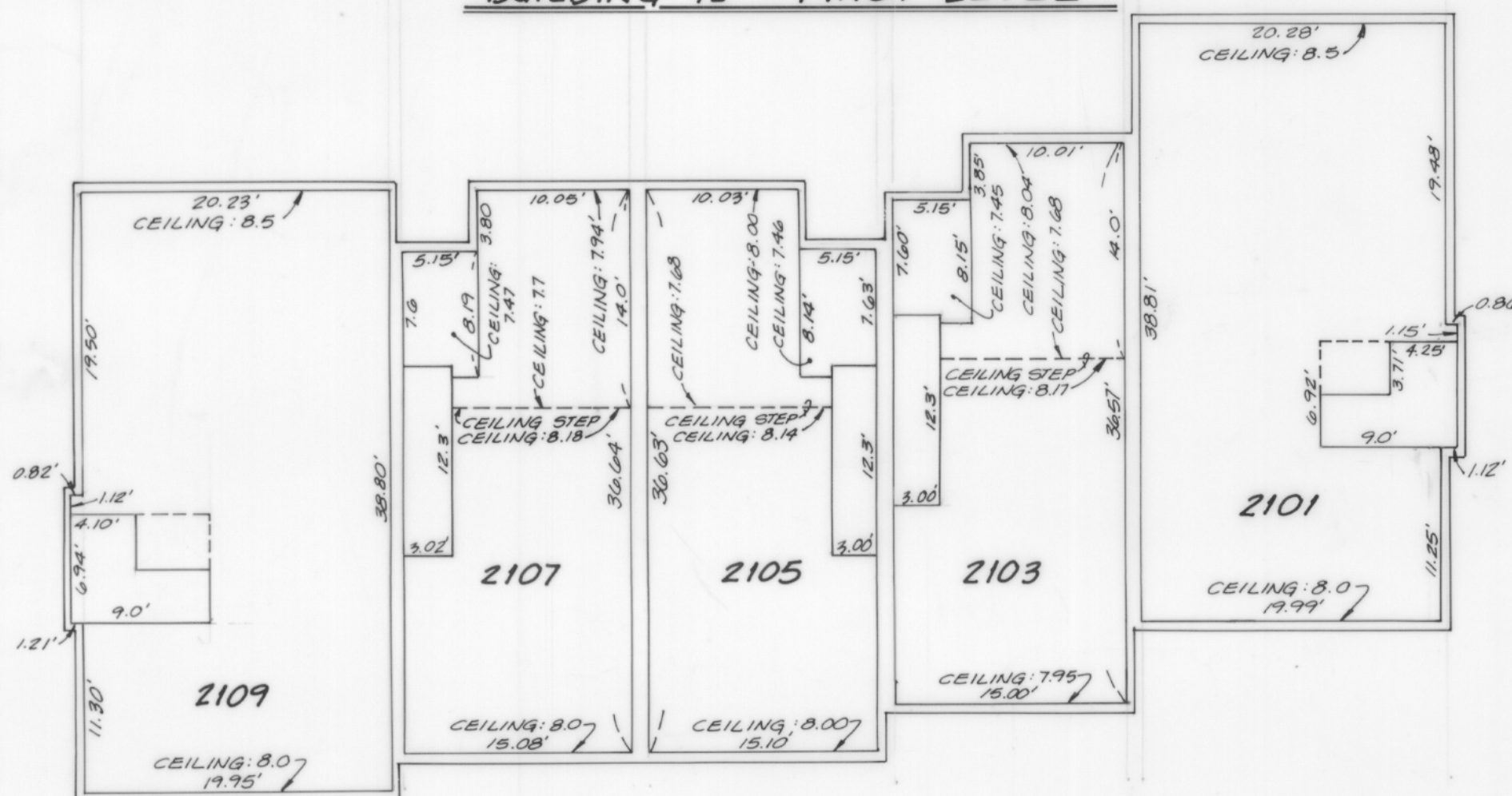
BUILDING '12' - GARAGE LEVEL
