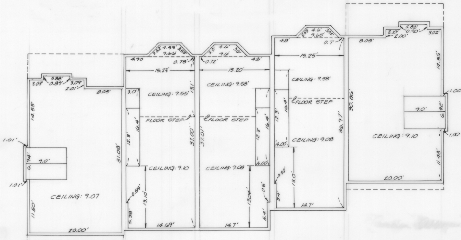
BUILDING '12' - FIRST LEVEL
