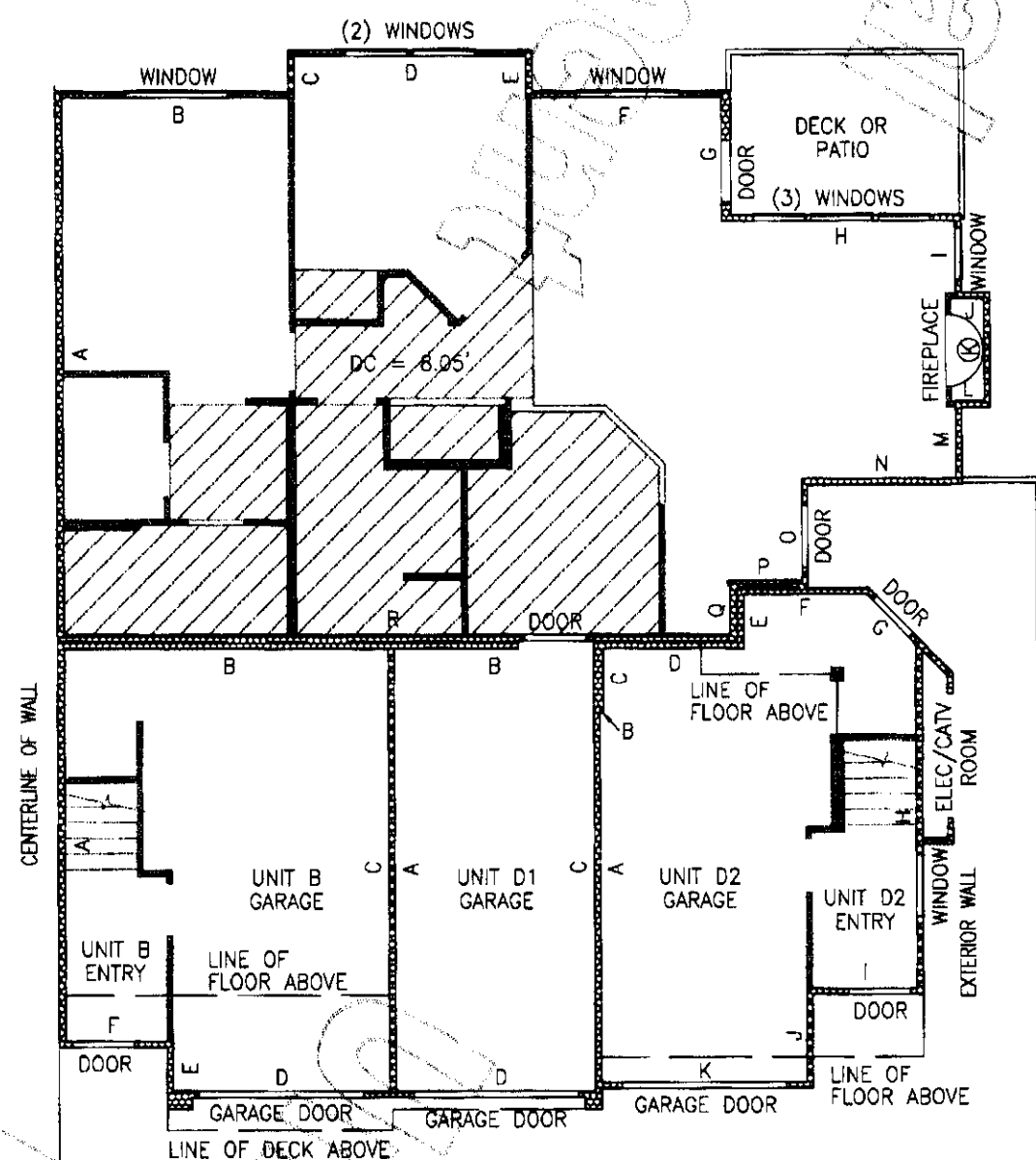
GARAGE PLAN
