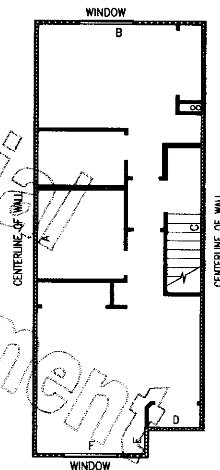
UNIT TYPE E SECOND FLOOR PLAN 1" = 8'
