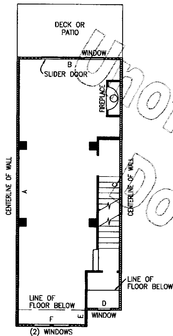
UNIT TYPE E FIRST FLOOR PLAN 1" = 8'
