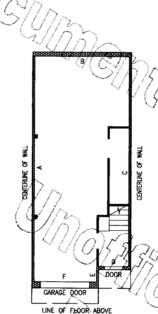
UNIT TYPE E BASEMENT 1" = 8'
