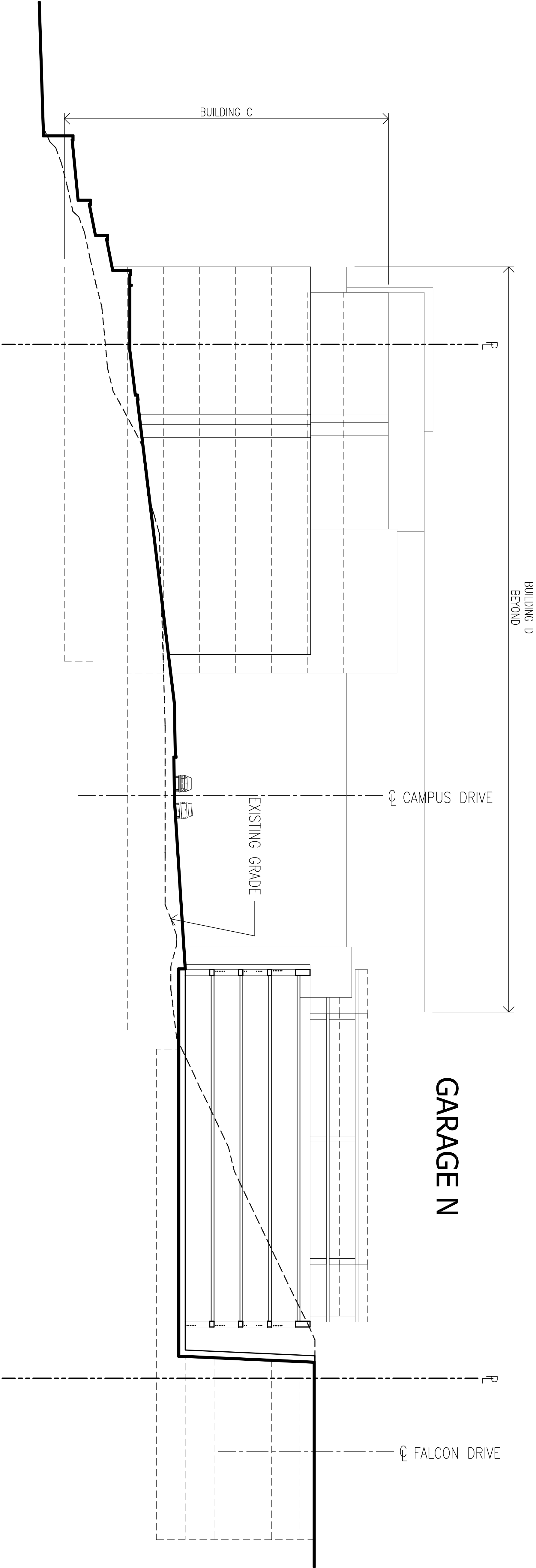
G-G SITE SECTION G-G 1" = 20'-0" 0 20' 40'
